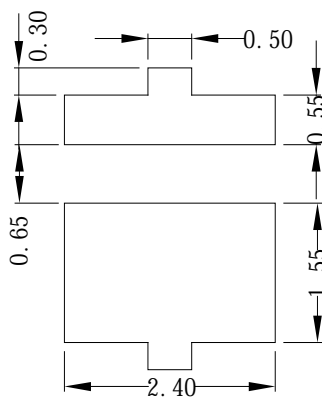
Fig.1-5 Soldering Patterns
