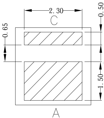
Fig.1-3 Bottom View
