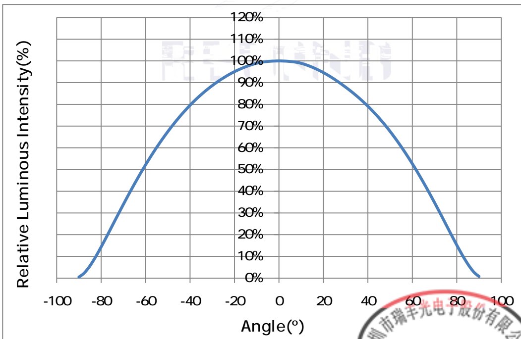
Fig. 1-12 Radiation diagram
