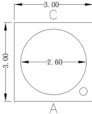
Fig.1-1 Top View
