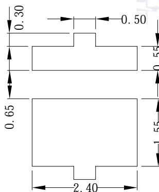
Fig.1-5 Soldering Patterns
