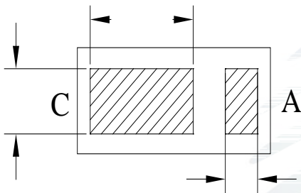
Fig. 1-3 Bottom View
