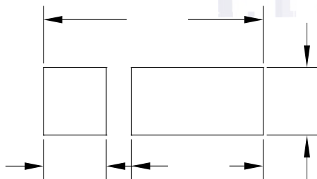
Fig. 1-5 Soldering Patterns
