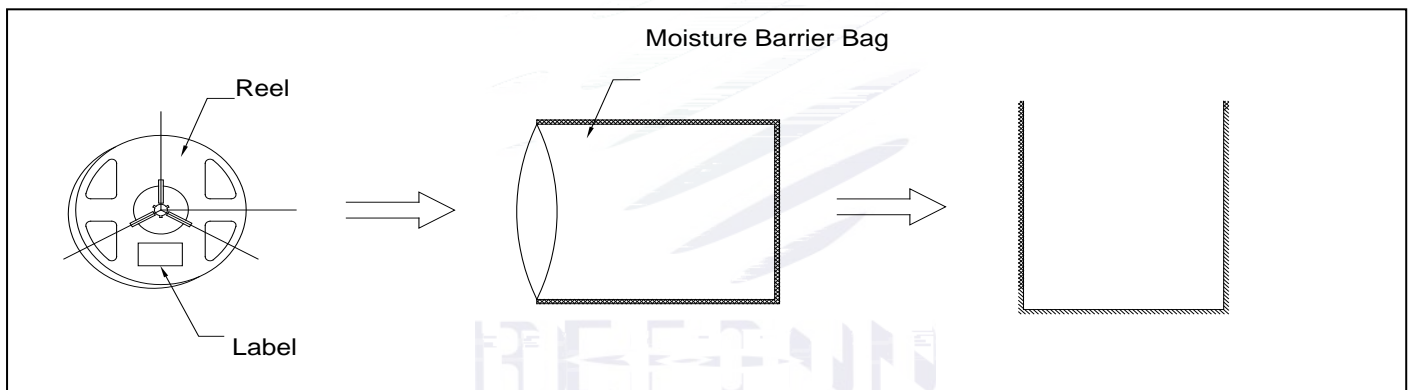
Fig.2-4Moisture Resistant Packing
