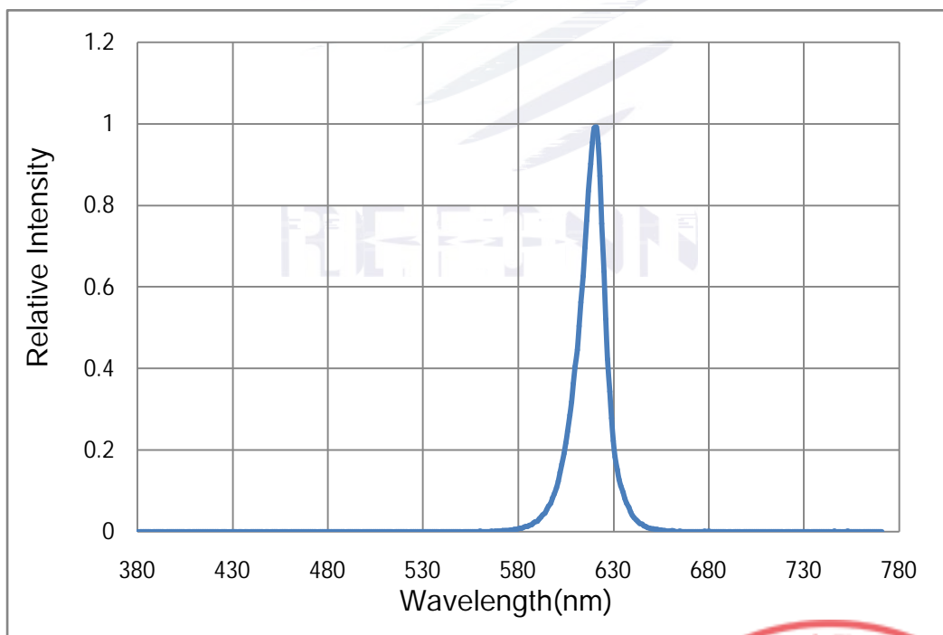
Fig. 1-14 Spectrum Distribution
