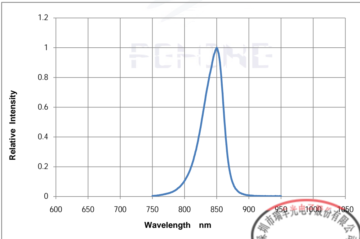
Fig. 1-14 Spectrum Distribution
