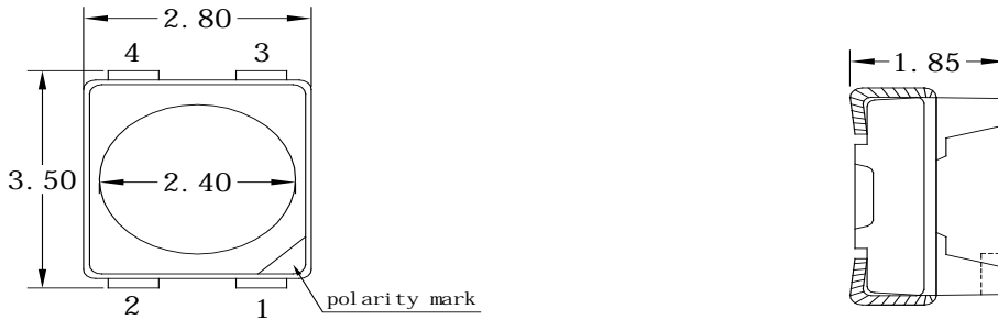
Fig. 1-1 Top View
