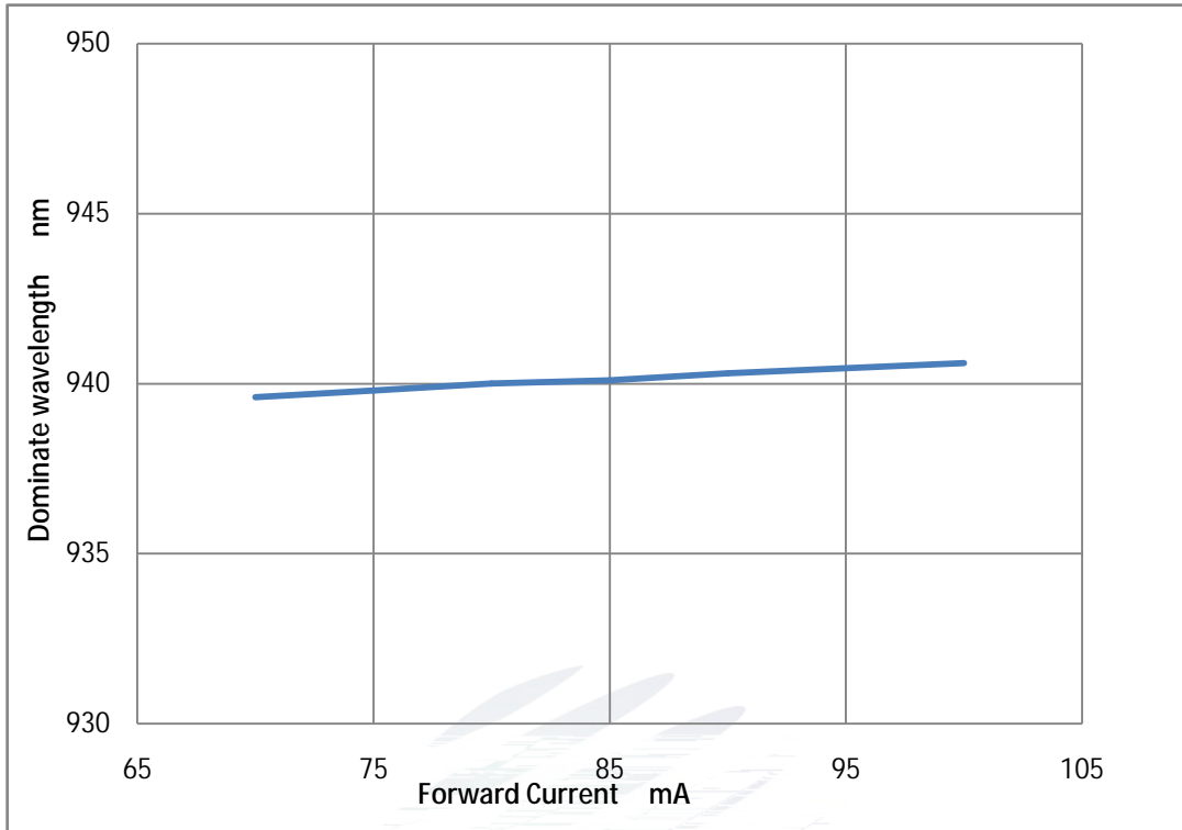
Fig. 1-13 Forward current vs. Dominate wavelength (Ts=25°C) (Ts=25°C)
