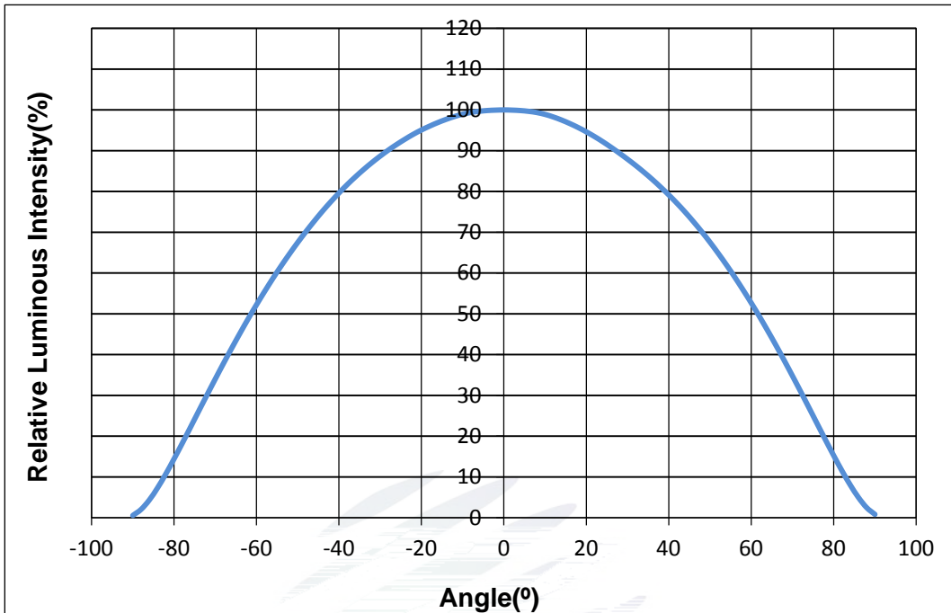
Fig. 1-13 Radiation diagram
