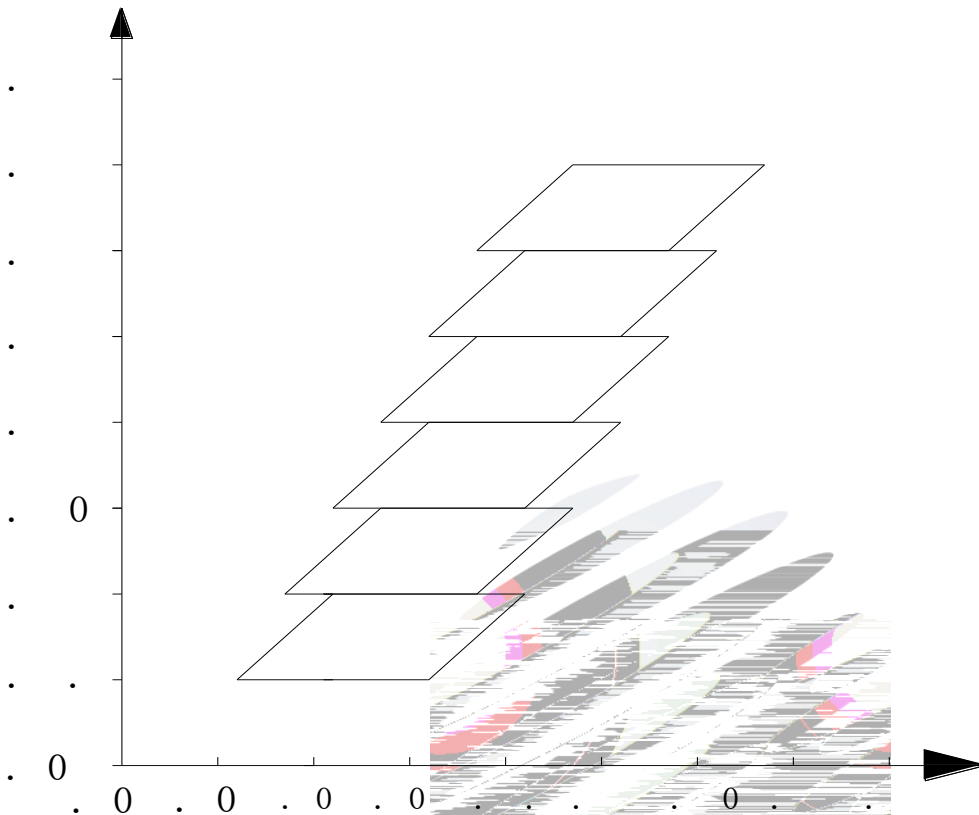
Fig. 1-6 The C.I.E Chromaticity Diagram CIE
