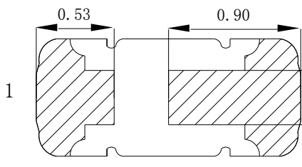
Fig.1-3 Bottom view
