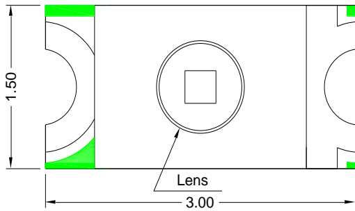
Fig.1-1 Top view
