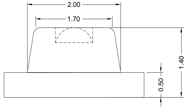
Fig.1-2 Side view
