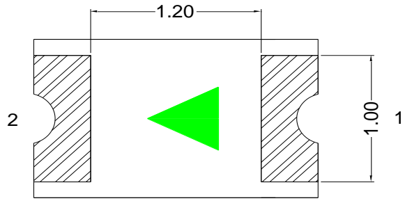
Fig.1-2 Bottom view
