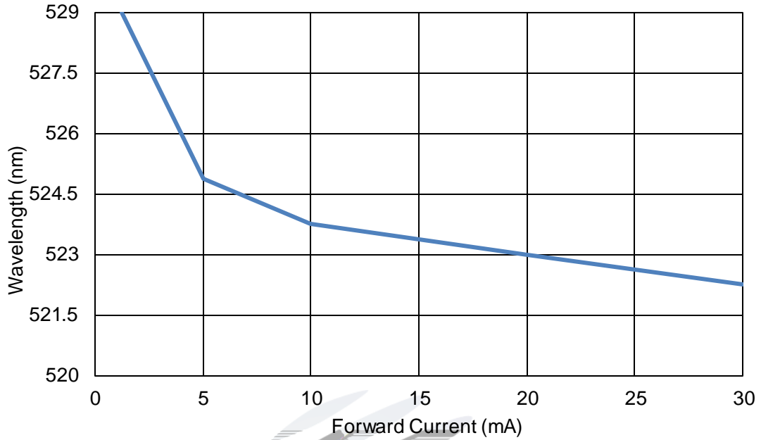
Fig 1-10 Forward Current Vs Dominate Wavelength (Ta=25°C)
