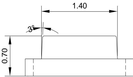
Fig.1-3 Side view
