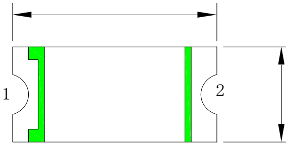
Fig.1-1 Top view
