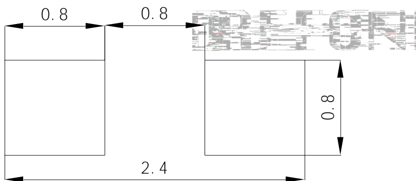
Fig.1-5 Soldering patterns
