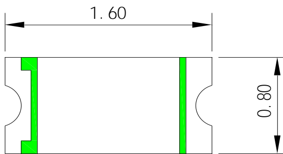
Fig.1-1 Top view
