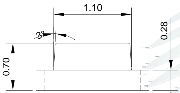
Fig.1-3 Side view
