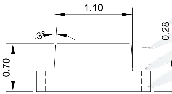
Fig.1-3 Side view
