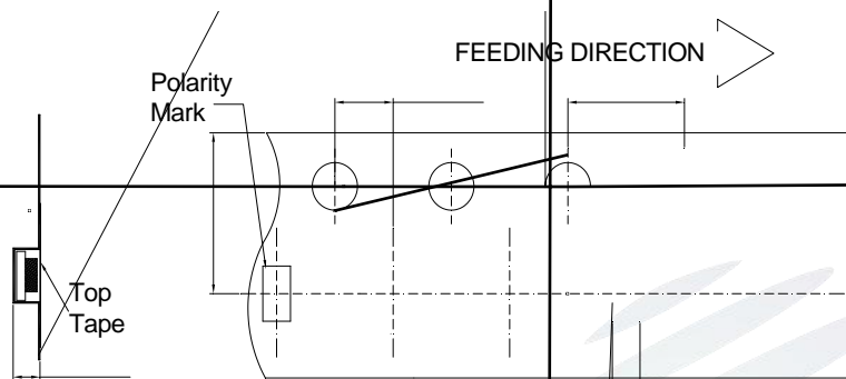
Fig.2-1 Carrier Tape Dimension
