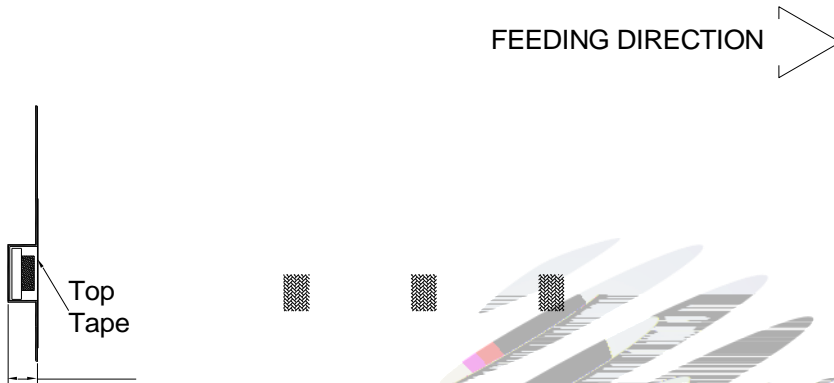
Fig.2-1 Carrier Tape Dimension
