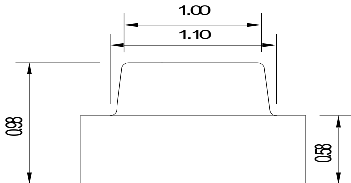
Fig.1-2 Side view
