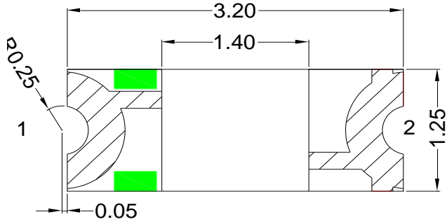
Fig.1-1 Top view
