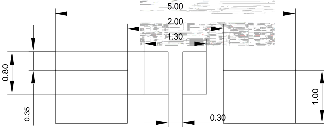
Fig.1-5 Soldering patterns
