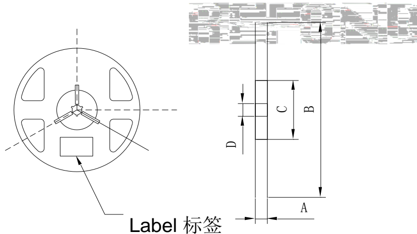
Fig.2-2 Reel Dimension
