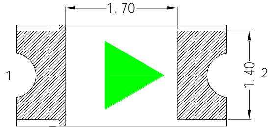
Fig.1-2 Bottom view
