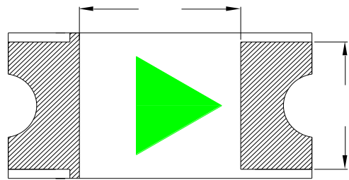
Fig.1-2 Bottom view
