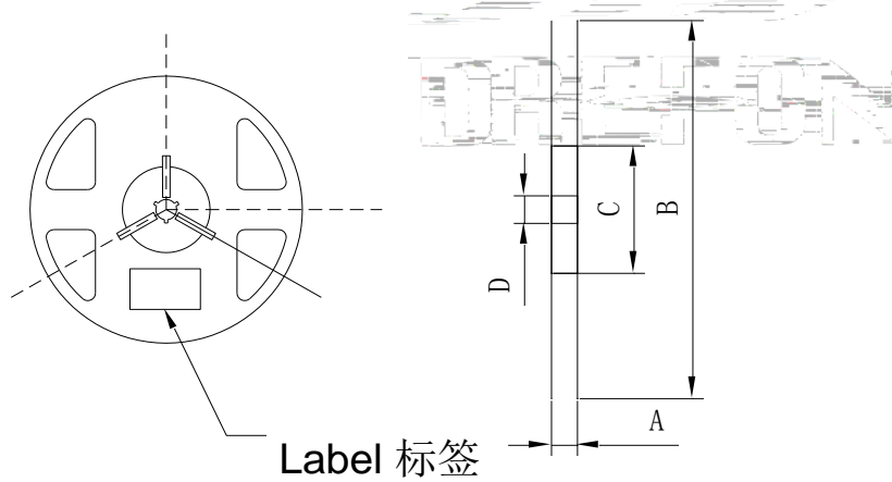
Fig.2-2 Reel Dimension
