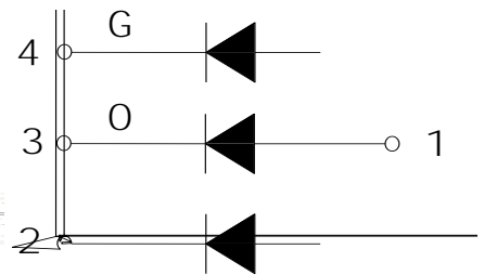
Fig.1-4 Polarity
