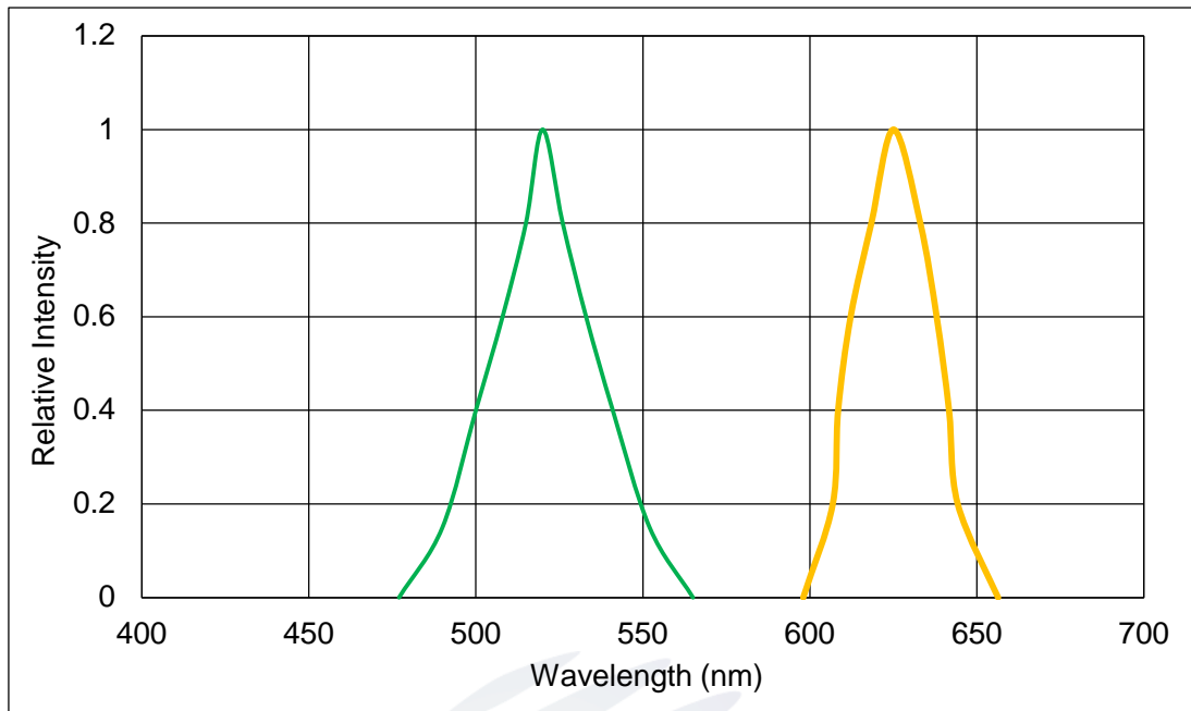
Fig.1-12 Relative Intensity Vs Wavelength ( T_a=25^{\circ}\text{C} )
