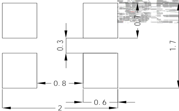
Fig.1-5 Soldering patterns
