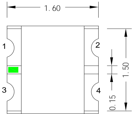
Fig.1-1 Top view
