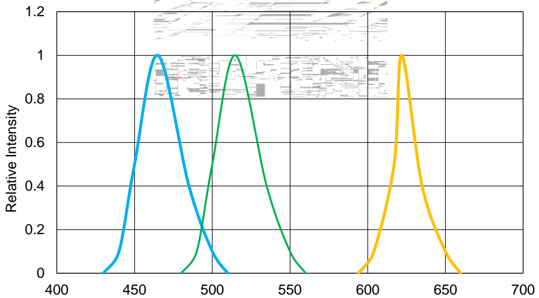
Fig.1-13 Relative Intensity Vs Wavelength (Ta=25°C)
