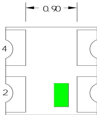
Fig.1-3 Bottom view
