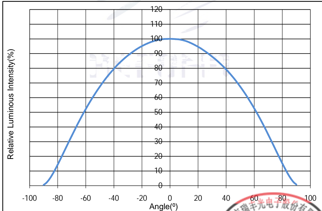
Fig. 1-12 Radiation diagram
