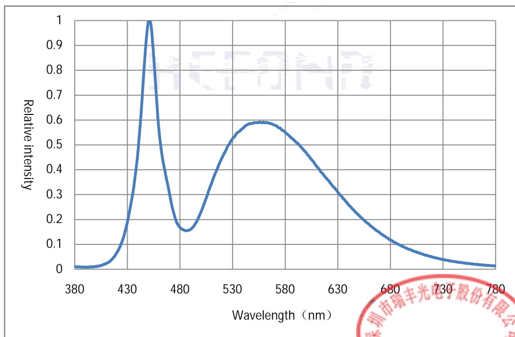
Fig. 1-14 Spectrum Distribution
