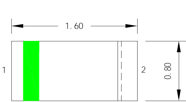
Fig.1-1 Top view
