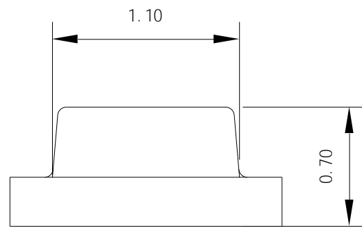
Fig.1-2 Side view
