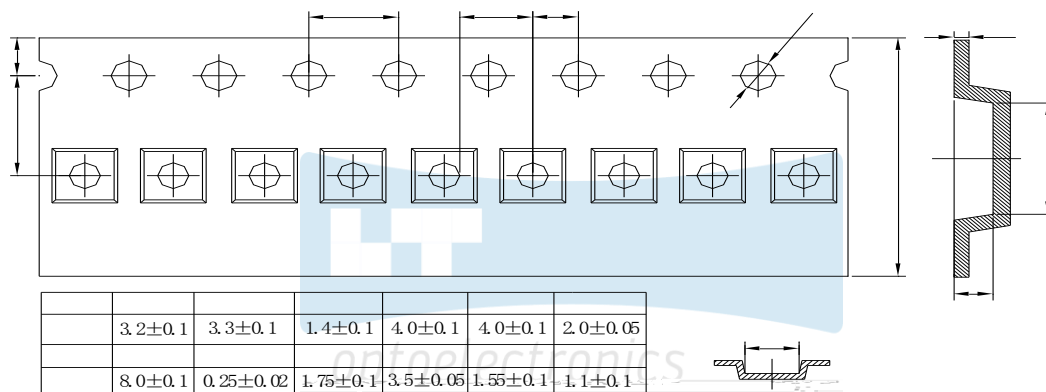
Fig 2-1 Carrier Tape Dimensions 载带尺寸
