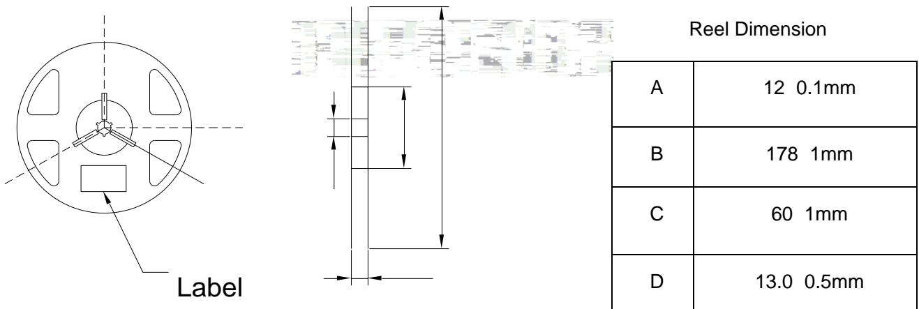
Fig.2-2 Reel Dimension
