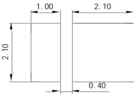
Fig.1-5 Soldering patterns
