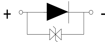
Fig.1-4 Polarity
