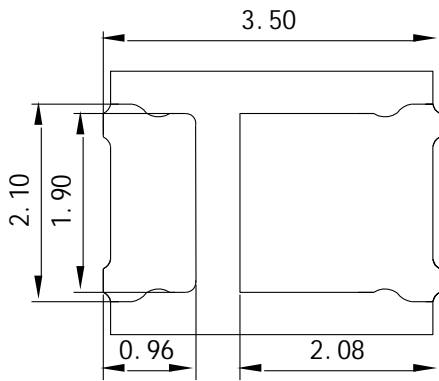
Fig.1-3 Bottom view
