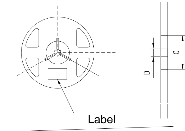
Fig.2-2 Reel Dimension
