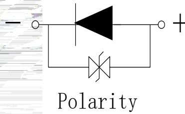
Fig.1-4 Polarity
