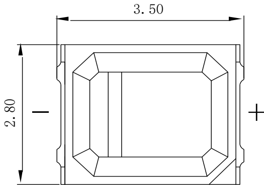
Fig.1-1 Top view
