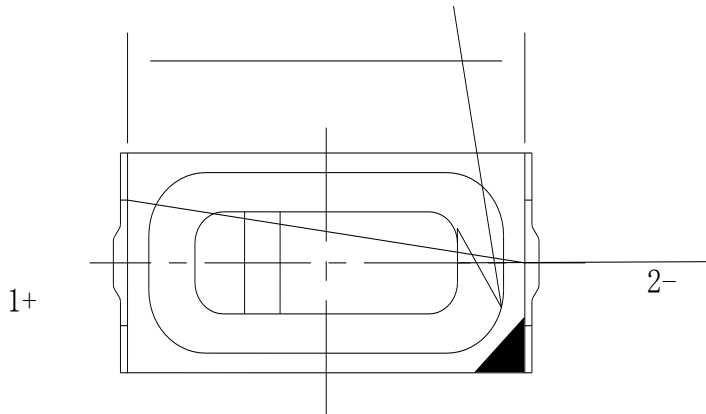
Fig.1-1 Top view
