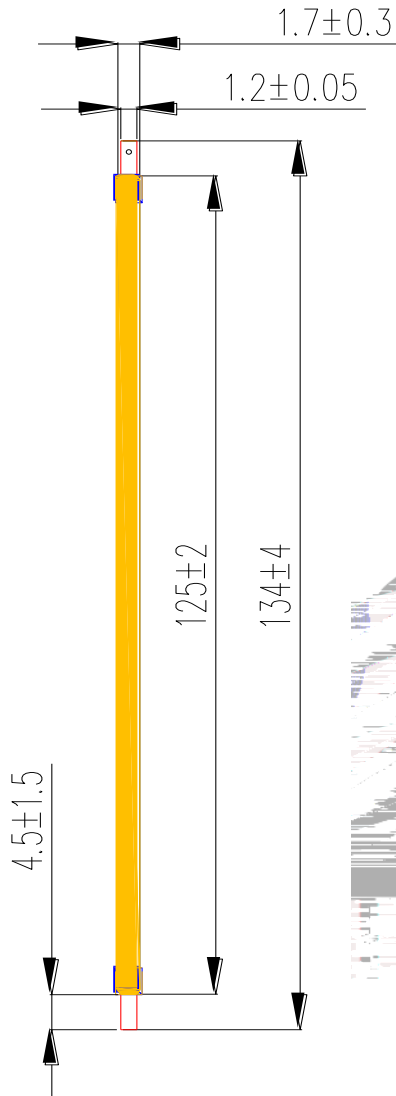
Fig.1-1 Top view
