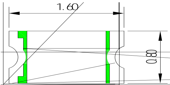
Fig.1-1 Top view
