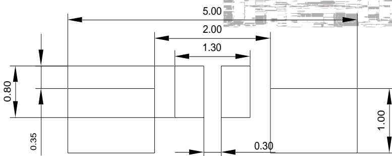
Fig.1-5 Soldering patterns
