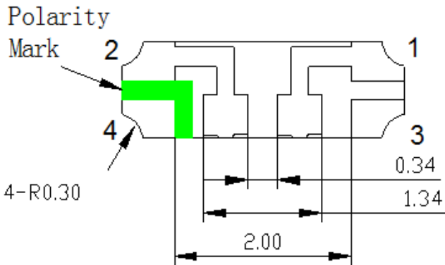
Fig.1-3 Bottom view
