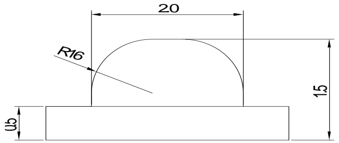
Fig.1-2 Side view
