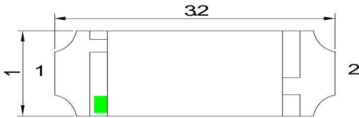
Fig.1-1 Top view
