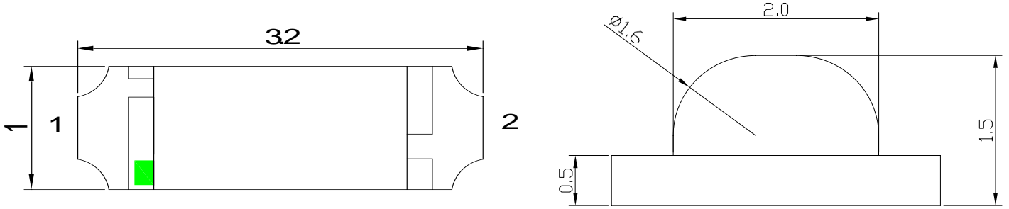
Fig.1-1 Top view
