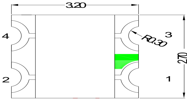
Fig.1-1 Top view
