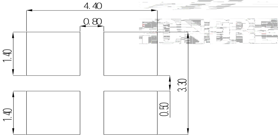
Fig.1-5 Soldering patterns
