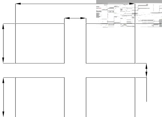
Fig.1-5 Soldering patterns
