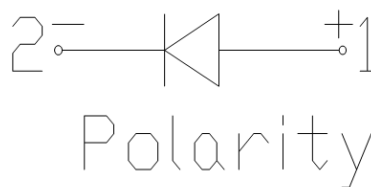
Fig.1-4 Polarity
