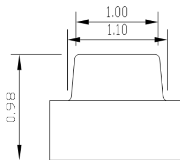
Fig.1-2 Side view
