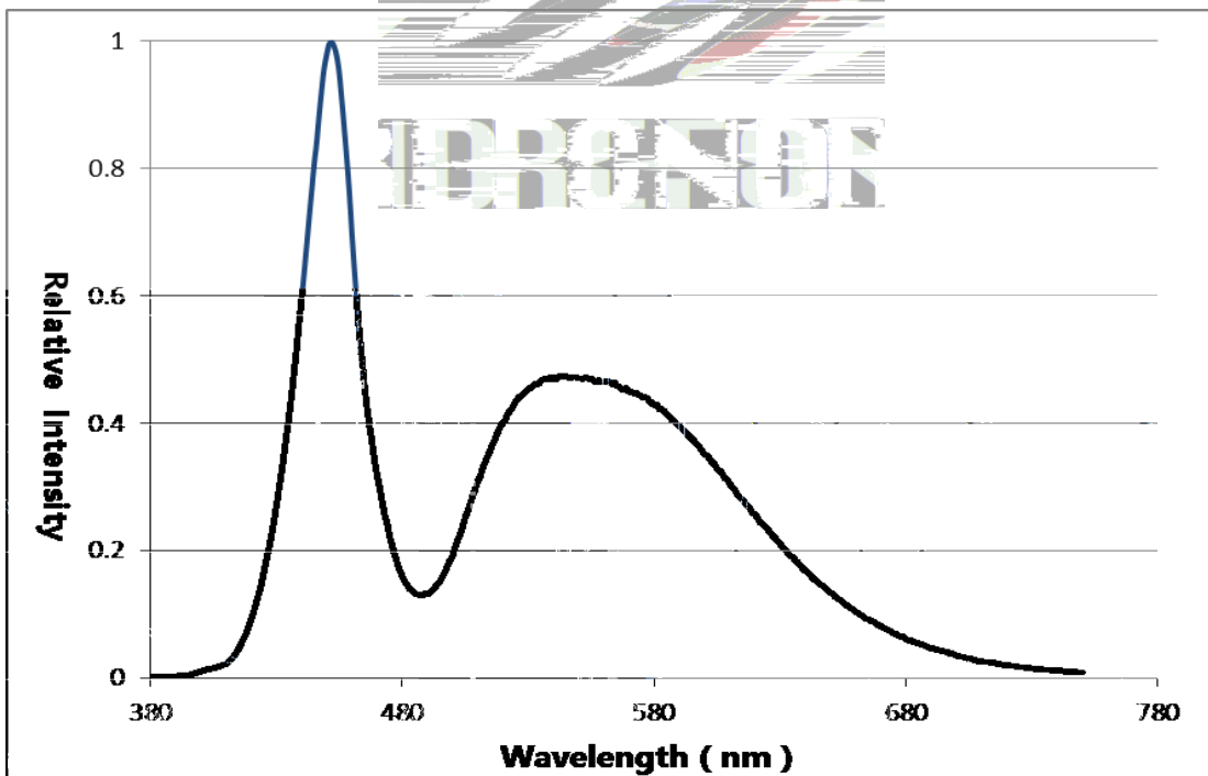
Fig. 1-14 Spectrum Distribution
