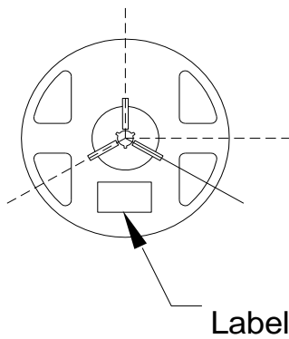
Fig.2-2 Reel Dimension
